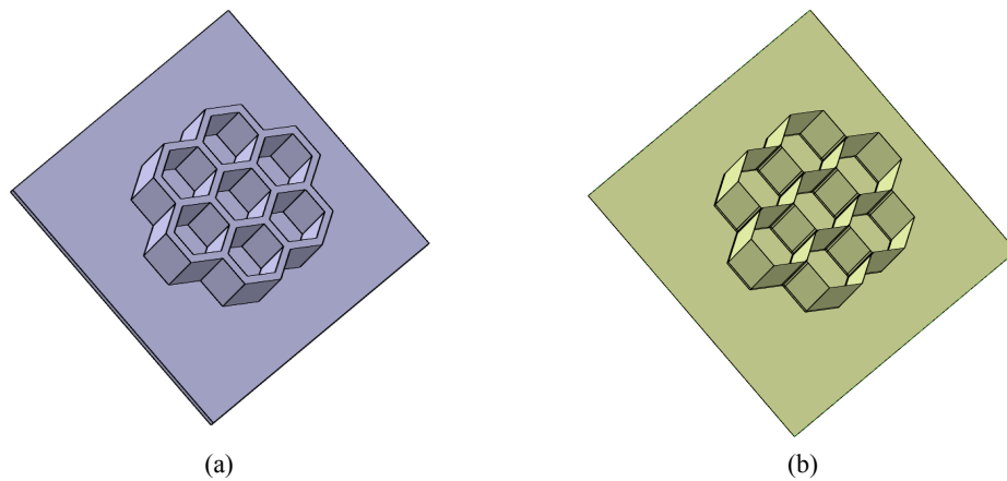
Fig. 18. Transformation from solid to mid-surface. (a) solid model and (b) mid-surface model.
