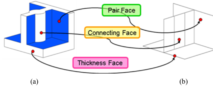
Fig. 10. Face relationship between models. (a) solid model and (b) surface model.
