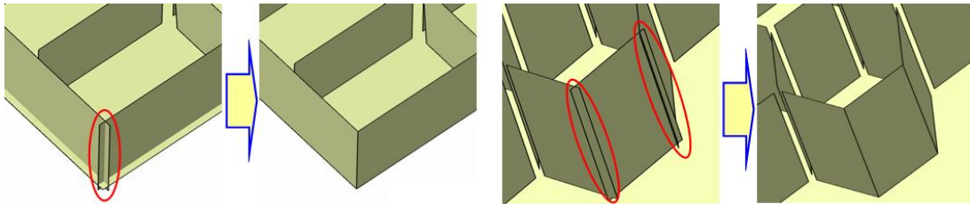
Fig. 13. Intersected patches and result of trimming operation.
