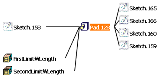
Fig. 6. ‘Parent-Child’ relationship.
