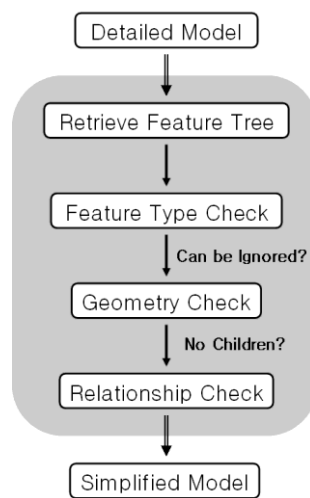
Fig. 5. Algorithm for simplification of detailed solid model.
