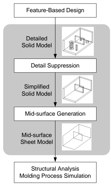
Fig. 2. Solid simplification and thinning processor for CAE model.
