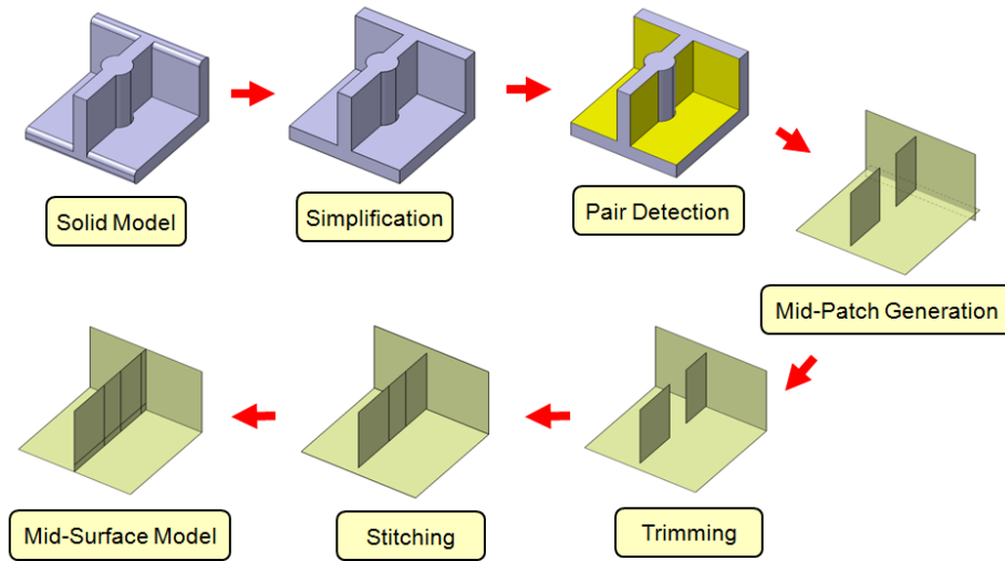
Fig. 4. Work flow for mid-surface model generation.
