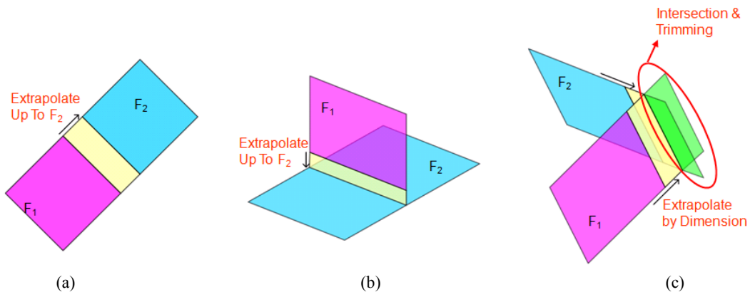
Fig. 15. Extending and stitching operation on (a) in-plane type, (b) T-joint type, and (c) L-joint Type
