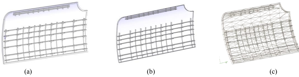
Fig. 1. Model Transformation. (a) solid model, (b) mid-surface model, and (c) mesh model for analysis.
