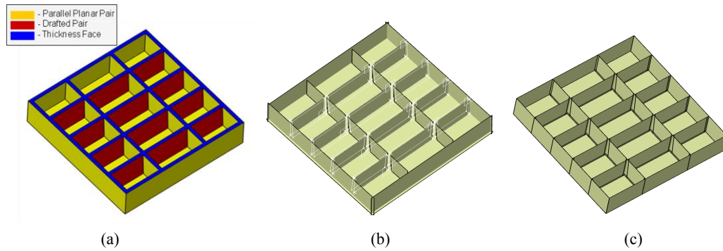
Fig. 17. Dimensional reduction process to mid-surface model. (a) face pair detection, (b) mid-patch generation, and (c) trimmed, extended, and stitched mid-surface model.
