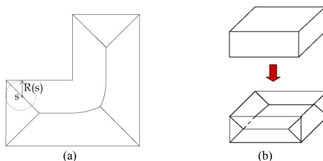
Fig. 3. Medial axis transform. (a) 2D MAT and (b) 3D MAT.
