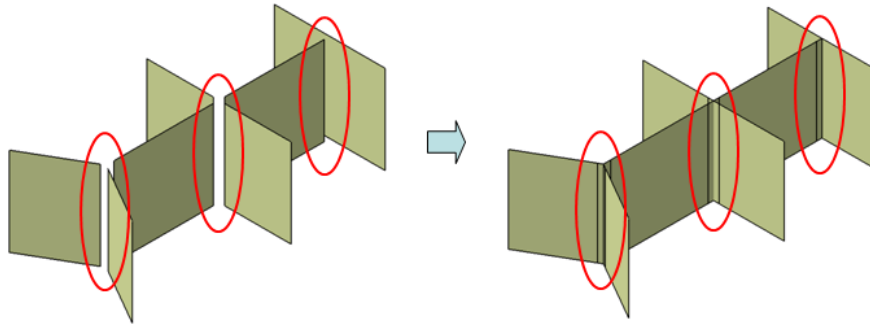
Fig. 14. Extending and stitching operation
